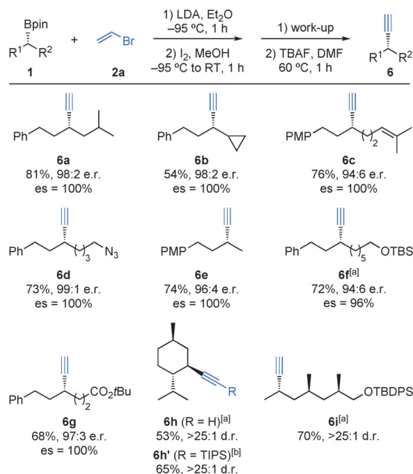
Scheme 2. Scope of alkynylation of secondary boronic esters. Reactions were carried out with 1 (0.30 mmol), 2a (1.0 M in THF, 0.60 mmol), LDA (0.86 M in THF, 0.60 mmol), I 2 (0.66 mmol), and TBAF·3 H 2 O (1.5 mmol). [a] LDA (0.86 M in THF, 0.75 mmol) was used instead of TBAF for dehydrobromination. [b] TIPSCl was added after dehydrobromination with LDA. The higher yield of 6h' was attributed to the volatility of 6h . TBAF = tetra- n -butylammonium fluoride; TBDPS = tert -butyldiphenylsilyl; TBS = tert -butyldimethylsilyl; TIPS = triisopropylsilyl; PMP = para -methoxyphenyl.
