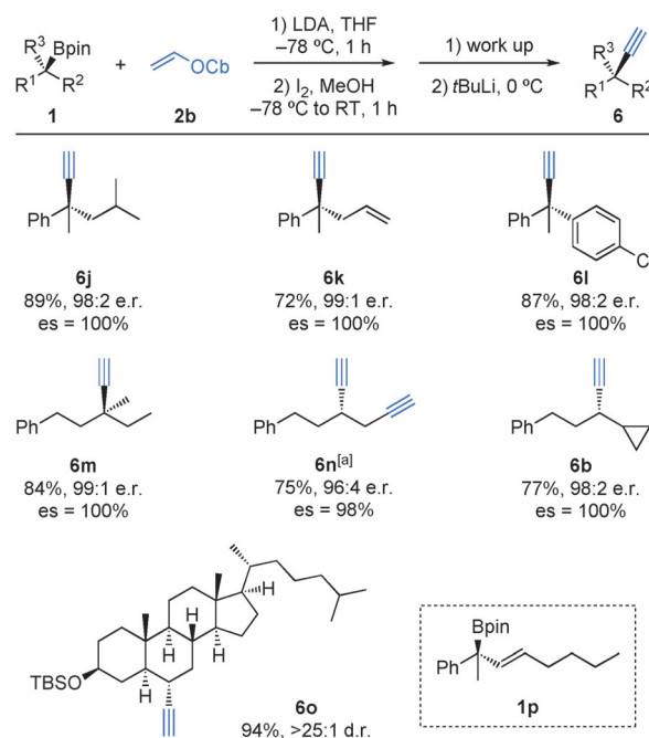
Scheme 4. Alkynylation of tertiary and hindered secondary boronic esters. Reactions were carried out with 1 (0.3 mmol), 2b (0.4 mmol), LDA (0.4 mmol), I 2 (0.4 mmol), and t BuLi (0.75 mmol). [a] 2b (1.2 mmol) and LDA (1.2 mmol) were used.
